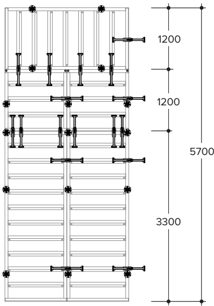
Formwork height: 5.70 m
