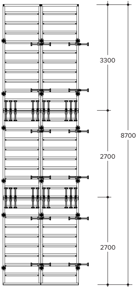
Formwork height: 8.70 m
