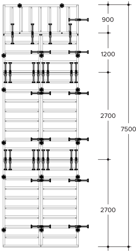
Formwork height: 7.50 m
