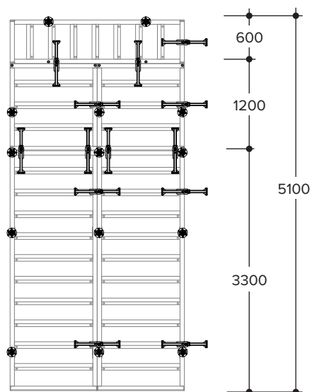
Formwork height: 5.10 m
