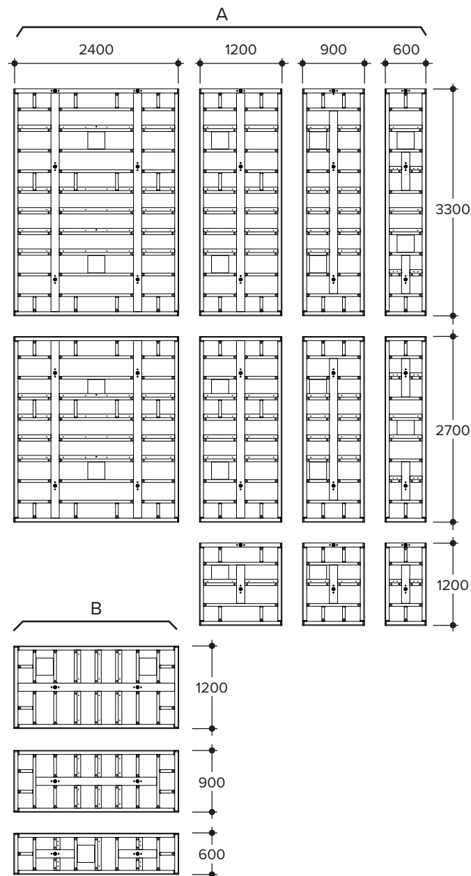
A - Panels; B - Extension panels.
