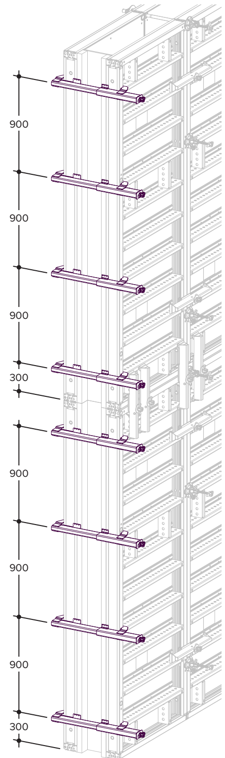
Panels 330, Hydrostatic and steady concrete pressure
