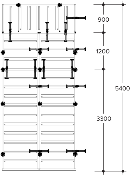
Formwork height: 5.40 m
