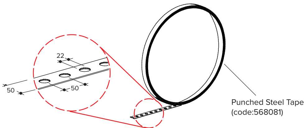
Punched Steel Tape (code:568081)
