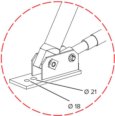
Strut Base
