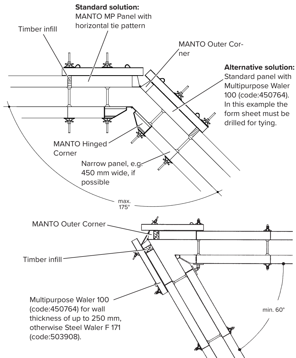
MANTO Hinged Corner
