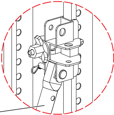
MANTO Strut Head (code:600035) to vertical panel
