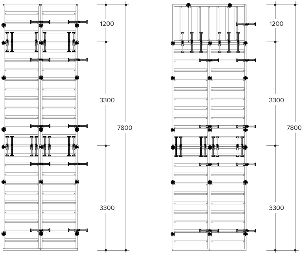
Formwork height: 7.80 m
