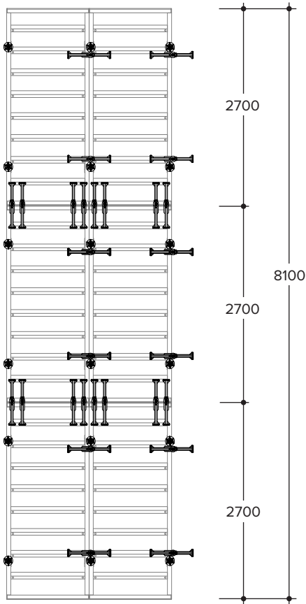
Formwork height: 8.10 m
