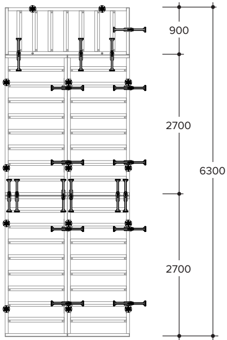
Formwork height: 6.30 m
