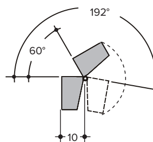
MANTO Outer Corner
