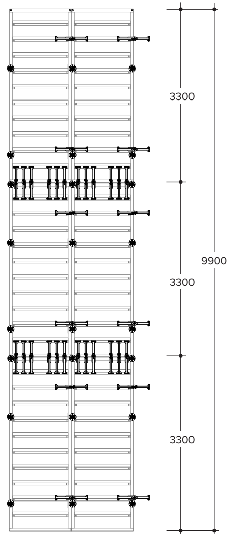
Formwork height: 9.90 m
