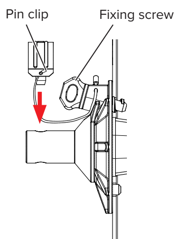
Fixing of the PLATINUM 100 Tie Nut Advancing Side
